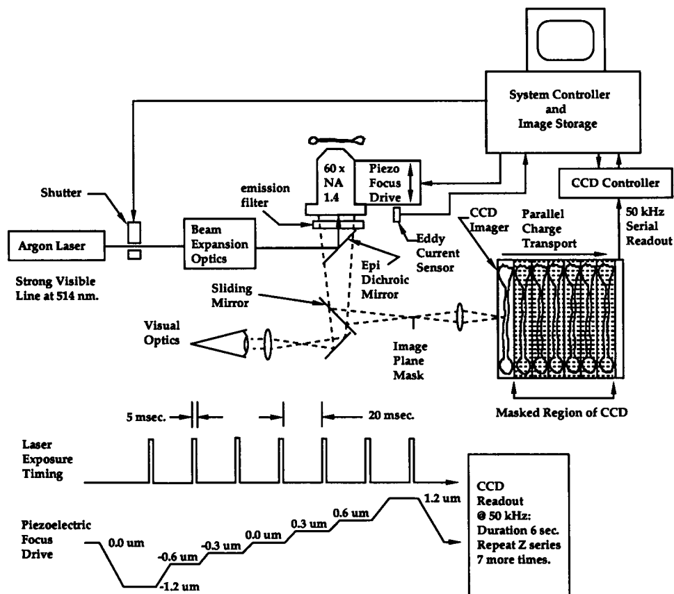
FIGURE 1 System and timing diagram of the fast 3D microscope. An argon laser (model 2025; Spectra Physics, Mountain View, CA) provides 250 mW of \lambda = 514 nm radiation. Exposures are timed by a fast shutter (Uniblitz, Rochester, NY; LS2 shutter and D122 driver). The laser beam is expanded and directed to the epi-illumination optics of a custom built inverted microscope, providing a widefield illumination flux of \sim 1 \times 10^{21} photons \text{cm}^{-2} \text{s}^{-1} at the specimen plane of the microscope. The fluorescent emission passes through a 550-nm longpass filter (Omega, Brattleboro, VT) and an intermediate image is formed by a plan apo 60 \times N.A.1.4 objective (Nikon, Garden City, NY). A mask placed in the plane of the intermediate image limits the field that is reimaged onto a 512 \times 512 pixel ccd camera (Photometrics, Tucson, AZ, model CC200 controller and CH250 camera head with Tektronix TK512 CCD). The imaged specimen field is \sim 10 \times 67 \mu\text{m} ( 73 \times 512 pixels, 130 \text{ nm/pixel} ). The masked area on the ccd is used to store up to 6 earlier images, which are shifted under the mask by parallel charge transport between exposures. At the same time, the focus is changed by a piezoelectric translator (model P-244.27 PZT and P-267 controller; Polytec Optonics, Costa Mesa, CA) attached to the center of mass of a counterweighted objective carrier. This drive configuration can attain stepped objective translations at rates of 1 \mu\text{m/ms} , but \sim 20 ms must be allowed for relaxation of the deformations introduced in the chamber coverslip by coupling of the objective motion through the immersion oil. Typical exposure times and focus positions are as illustrated. After the ccd is filled with a 7-image through-focus series, the ccd is read out ( \sim 6 s) and the process repeated to obtain a time series.
