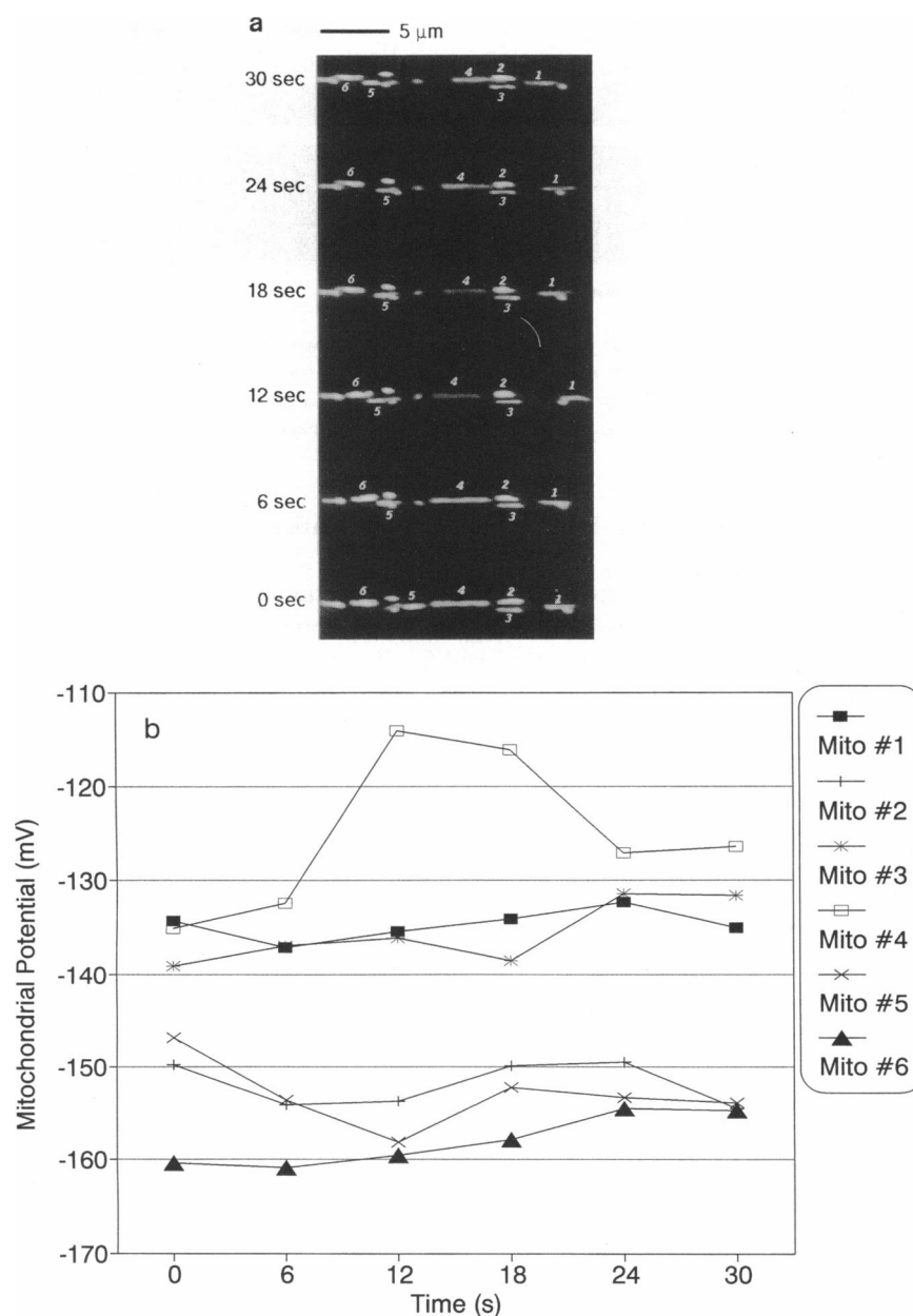
FIGURE 7 Mitochondria occasionally display large membrane potential fluctuations. (a) Time series of restored images taken at 6-s intervals. Notice the loss of intensity in mitochondrion 4 in the 3rd and 4th time points. (b) V_{mit} is plotted for each of the labeled mitochondria, indicating the magnitude of the fluctuation in mitochondrion 4.
