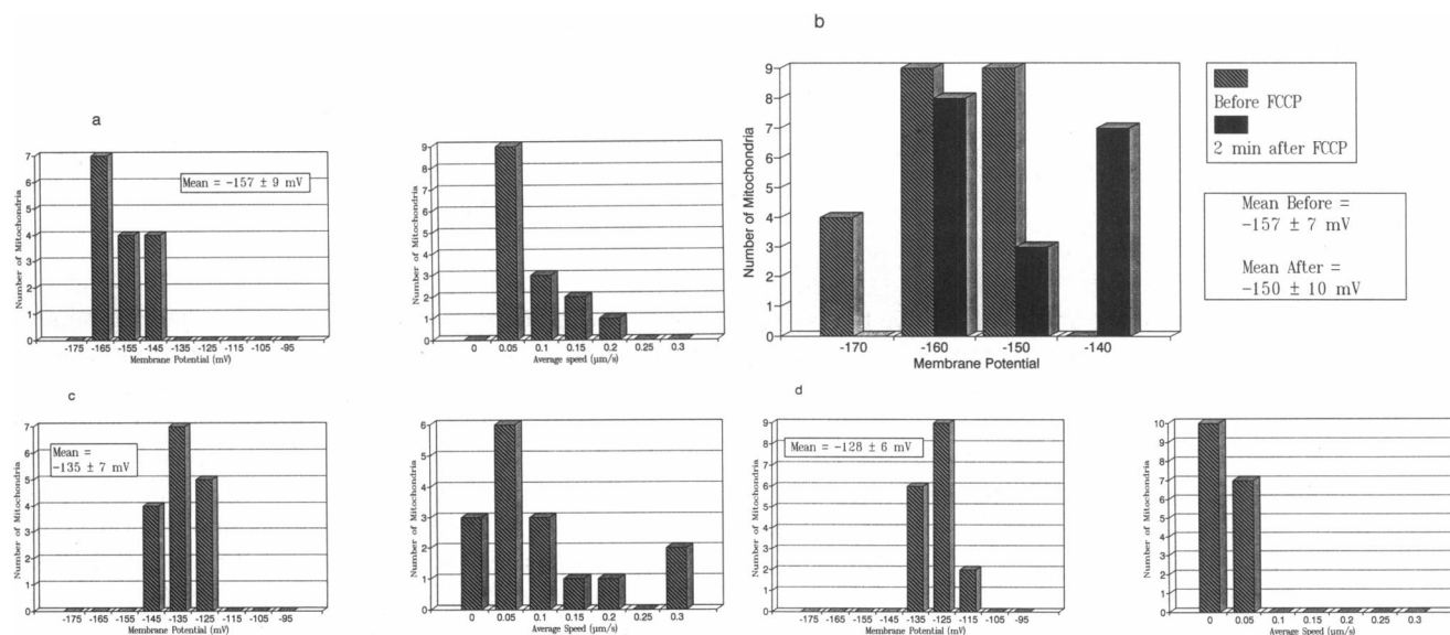
FIGURE 9 Mitochondrial potential is depolarized to a new level by an uncoupler. Cells were mounted on the thermostatted chamber and imaged before and after introduction of medium containing 0.1 \mu\text{M} FCCP. After restoration, V_{\text{mit}} was calculated according to Eq. 3; in addition, the cartesian coordinates of the centroids of each mitochondrion in a 42-s time series of 8 3D images was used to calculate the average speed of the individual mitochondria. All data were obtained from neurites on a single coverslip, but, because phototoxic effects became evident after too much light exposure, several neurites had to be sampled. ( a ) Histograms of V_{\text{mit}} and speed distributions from a neurite before FCCP treatment. ( b ) Histograms of V_{\text{mit}} from the same neurite before and 2 min after treatment with 0.1 \mu\text{M} FCCP. ( c ) Potential and motion histograms in a third neurite 5 min after 0.1 \mu\text{M} FCCP. ( d ) A fourth neurite, 28 min later, displays a stable potential but a loss of saltatory motion.
