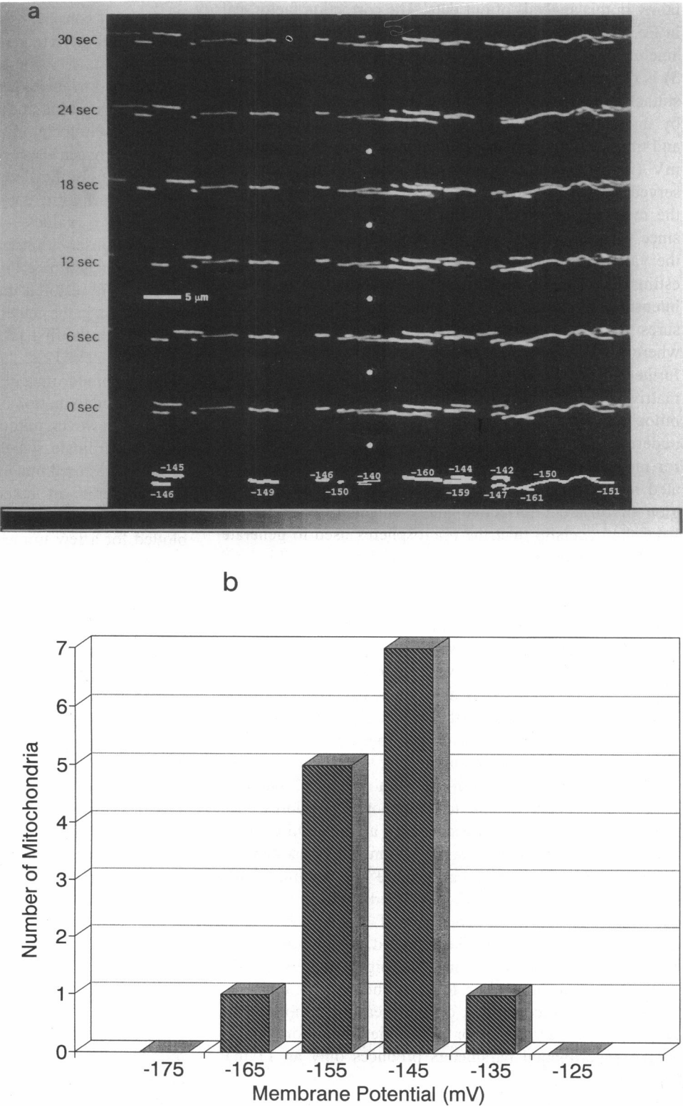
FIGURE 6 Assignment of membrane potentials to motile mitochondria. ( a ) An experiment in which individual mitochondria have been analyzed. The bottom image indicates the membrane potentials of each analyzed mitochondrion. A time sequence of projections of the 3D datasets onto a single plane is displayed above with times, in seconds, indicated. Saltatory motion of the mitochondria is evident. A fluorescent calibration bead is seen toward the center of each image; its intensity saturates the display, which was scaled to best visualize the mitochondria, but is within the range of the 16-bit image. ( b ) Histogram of membrane potentials in individual mitochondria from the initial time point of the neurite in a .
